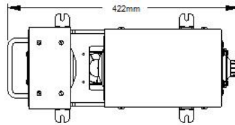
Sealing Head With Safety Shield Open & Closed See dimensional drawings below, Weight 9.1 Kg
